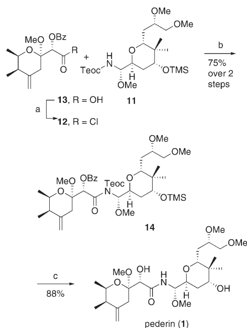
Scheme 3. Synthesis of pederin: a) \text{SOCl}_2 , pyridine, \text{CH}_2\text{Cl}_2 , RT; b) LiHMDS, THF, -78^\circ\text{C} to RT; c) TBAF, THF, 0^\circ\text{C} , LiOH/MeOH quench. Bz = benzoyl, TBAF = tetra- n -butylammonium fluoride.
