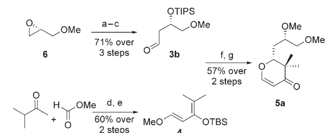
Scheme 1. Synthesis of 5a : a) vinyl Grignard reagent, CuI, THF, −78 °C to 0 °C; b) TIPS-Cl, imidazole, CH 2 Cl 2 ; c) O 3 , CH 2 Cl 2 ; PPh 3 quench; d) NaOMe, Et 2 O, reflux; DMSO, Me 2 SO 4 ; e) TBSOTf, Et 3 N, Et 2 O, 0 °C to RT; f) Al(2,6-diphenylphenoxide) 2 Me (0.4 equiv), TMSOTf (2.1 equiv), CH 2 Cl 2 , −78 °C to −45 °C; 10% HF/MeCN quench; g) NaHMDS, MeI, THF, −78 °C to 0 °C. DMSO = dimethyl sulfoxide, HMDS = hexamethyldisilazane.
